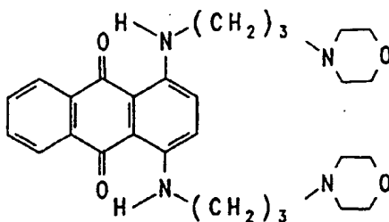
Compound 1c
